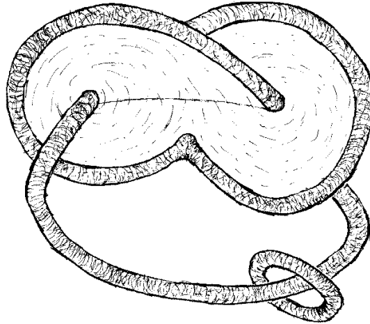
Fig. 8. Lorenz-Smale flow with a trefoil attractor is a left or right handed trefoil. See [2, Lemma 15.37, Corollary 15.23].
