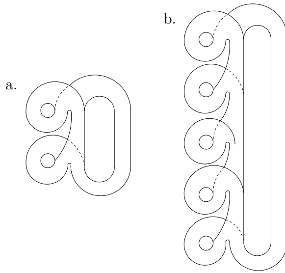
Fig. 14. Two templates containing all knots
