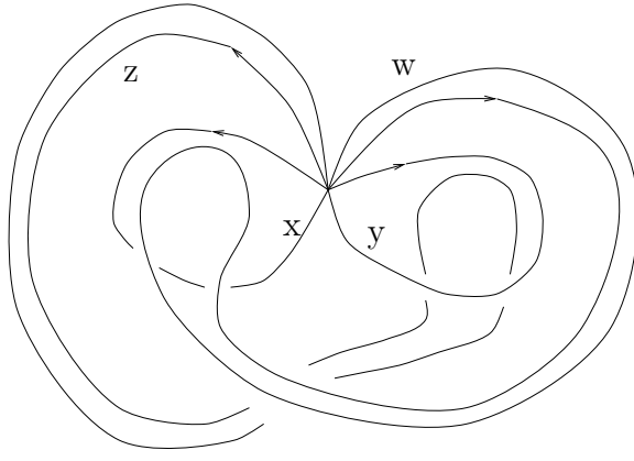
Fig. 9. The generators of \pi_1(R \cap L) and \pi_1(L) .
