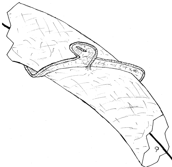
Fig. 6. y is a (p, q) cable of a
