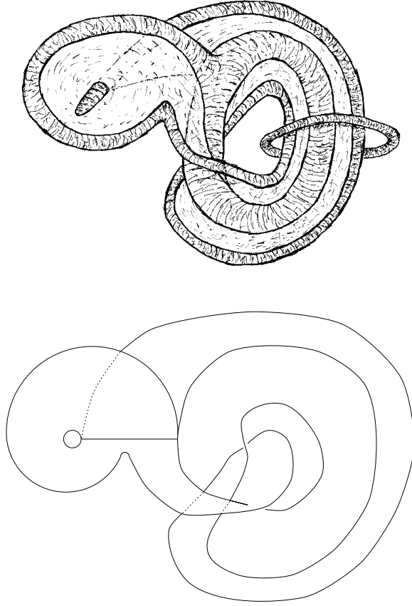
Fig. 7. The top figure has an attractor in the fat tube and a repeller in the thin tube. A template for the saddle set is shown below. The loop y is a (2,1) torus curve. Any (p,q) torus curve, knotted or unknotted, can be realized.
