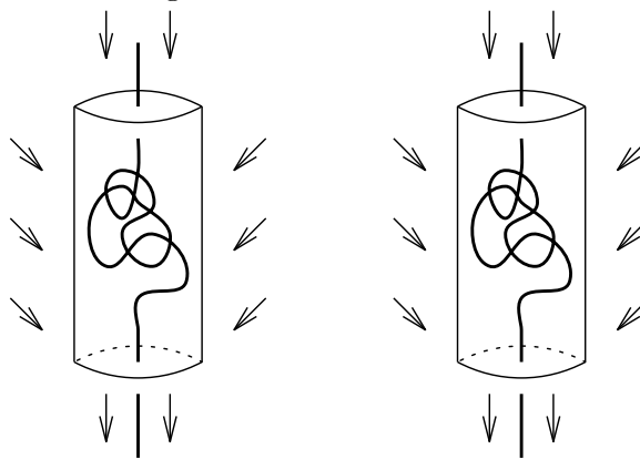
Fig. 12. Cut out these balls.
