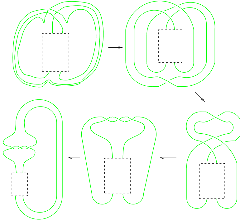
Fig. 11. \gamma is a satellite of \alpha
