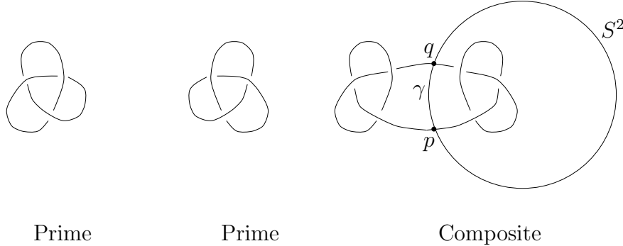
Fig. 2. The square knot is the sum of two trefoils.
