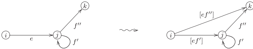
FIGURE 1. A basic positive equivalence.
