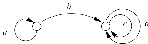
FIGURE 1. Graph for Example 2.1
