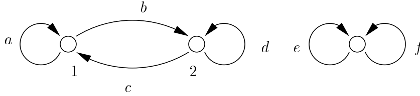
FIGURE 2. These SFTs are topologically equivalent.
