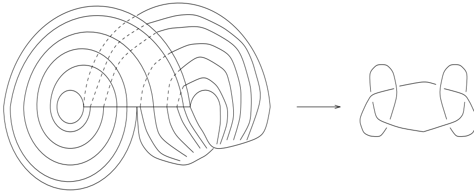
FIGURE 2. A square knot in L(0, -1)
