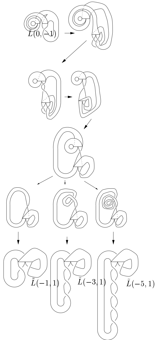
FIGURE 9. Rest of Theorem 3
