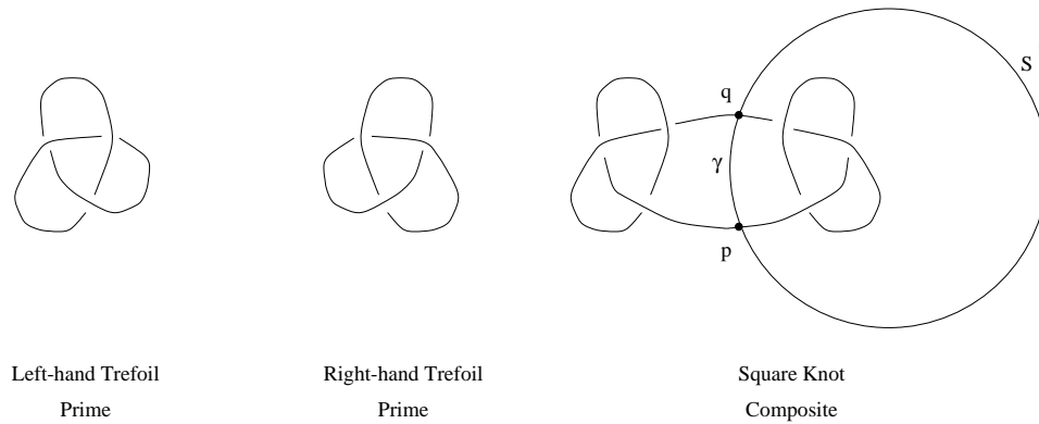
FIGURE 3. A connected sum
