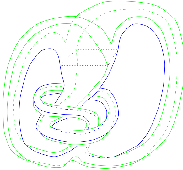
Fig. 10. The gray curve is \gamma .
