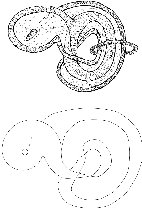
Fig. 7. The top figure has an attractor in the fat tube and a repeller in the thin tube. A template for the saddle set is shown below. The loop y is a (2,1) torus curve. Any (p, q) torus curve, knotted or unknotted, can be realized.
