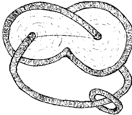
FIGURE 1.2: Smale flow with three basic sets
