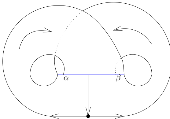
FIGURE 1.4: Geometric Lorenz Attractor
